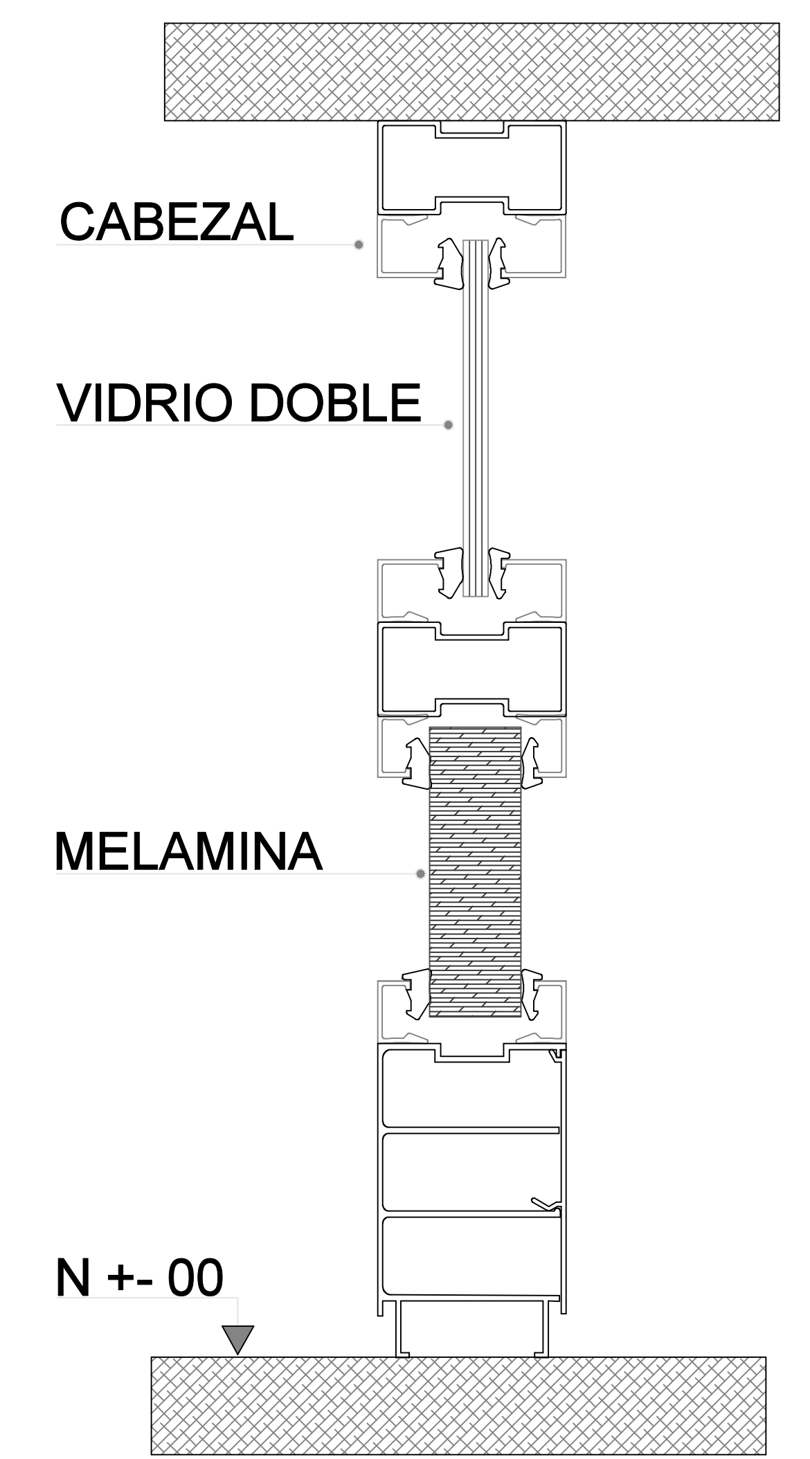
CORTE VERTICAL
